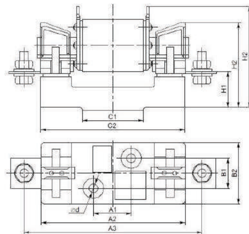
ДП-35, ДП-37, ДП-39
